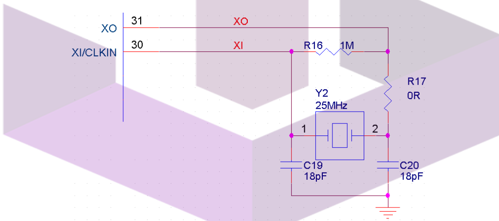
Figure 3. Crystal reference schematic
