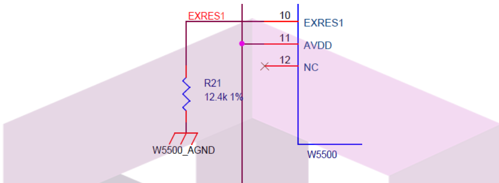
Figure 2. External reference resistor
