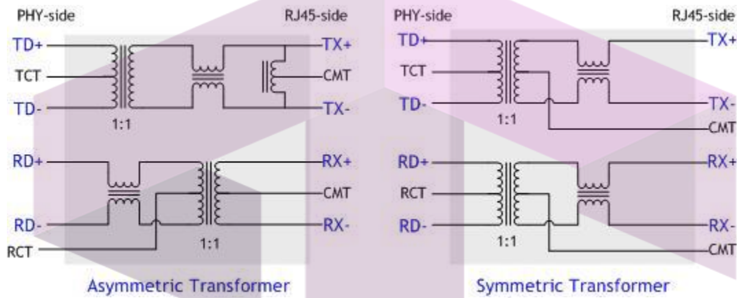
Figure 24. Transformer Type
