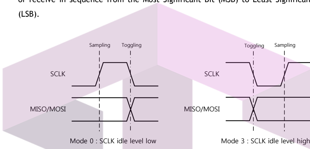
Figure 6. SPI Mode 0 & 3
